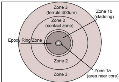
Ferrule Inspection Standard
